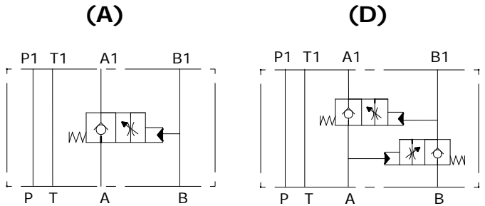
Schema idraulico Hydraulic diagram
